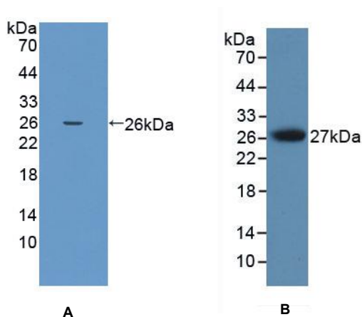
Figure 1. Western Blot
