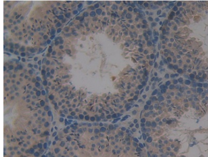
DAB staining on IHC-P; Samples: Mouse Testis Tissue; Primary Ab: 10µg/ml Rabbit Anti-Mouse PKD1 Antibody Second Ab: 2µg/mL HRP-Linked Caprine Anti-Rabbit IgG Polyclonal Antibody (Catalog: SAA544Rb19)
