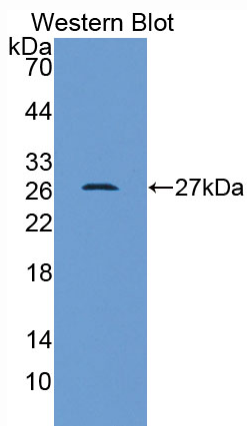
Used in Western Blot, Sample: Recombinant RAD54L2, Human
