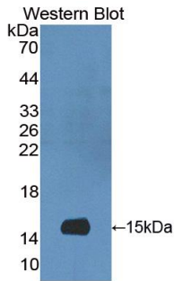
Figure. Western Blot; Sample: Recombinant S100A9, Bovine.
