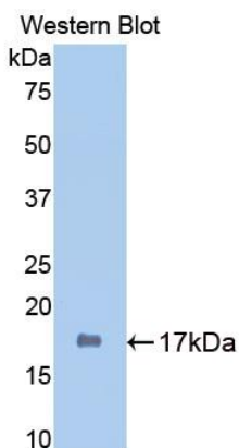
Used in Western Blot, Sample: Recombinant SIRT7, Rat
