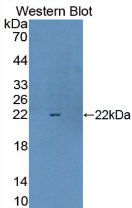
Used in Western Blot, Sample: Recombinant Surv, Human
