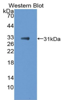
Figure. Western Blot; Sample: Recombinant TBX21, Mouse.
