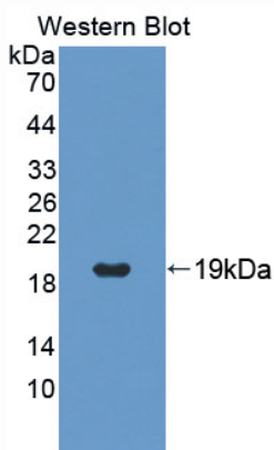
Used in Western Blot, Sample: Recombinant TIAM1, Human
