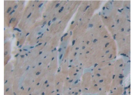
DAB staining on IHC-P; Samples: Mouse Heart Tissue; Primary Ab: 40µg/ml Rabbit Anti-Mouse TFR2 Antibody Second Ab: 2µg/mL HRP-Linked Caprine Anti-Rabbit IgG Polyclonal Antibody (Catalog: SAA544Rb19)
