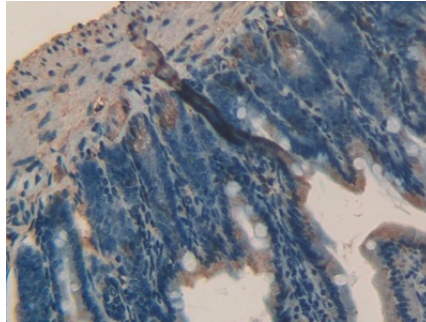
DAB staining on IHC-P; Samples: Mouse Intestine Tissue; Primary Ab: 40µg/ml Rabbit Anti-Mouse TFR2 Antibody Second Ab: 2µg/mL HRP-Linked Caprine Anti-Rabbit IgG Polyclonal Antibody (Catalog: SAA544Rb19)
