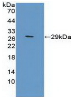
Figure. Western Blot; Sample: Recombinant TFR2, Mouse.
