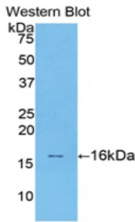
Figure. Western Blot; Sample: Recombinant TGFb1, Rat.
