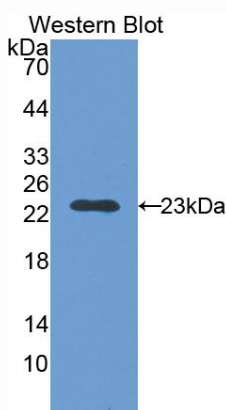
Used in Western Blot, Sample: Recombinant TNNI1, Rat
