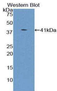
Figure. Western Blot; Sample: Recombinant UGT8, Human.
