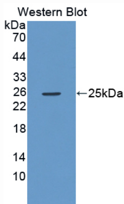
Used in Western Blot, Sample: Recombinant UPP1, Human
