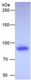
Figure. SDS-PAGE
