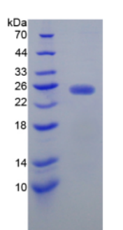
Figure. SDS-PAGE
