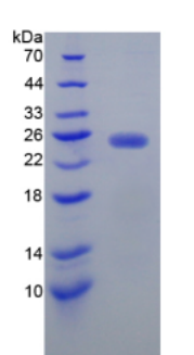
Figure. SDS-PAGE
