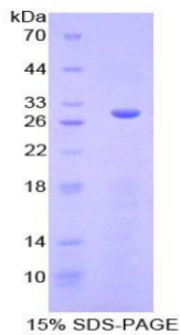
Figure. SDS-PAGE
