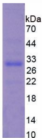
Figure 1. SDS-PAGE
