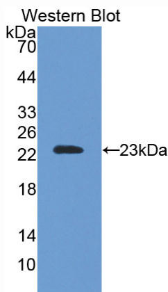
Used in Western Blot, Sample: Recombinant SOD2, Mouse
