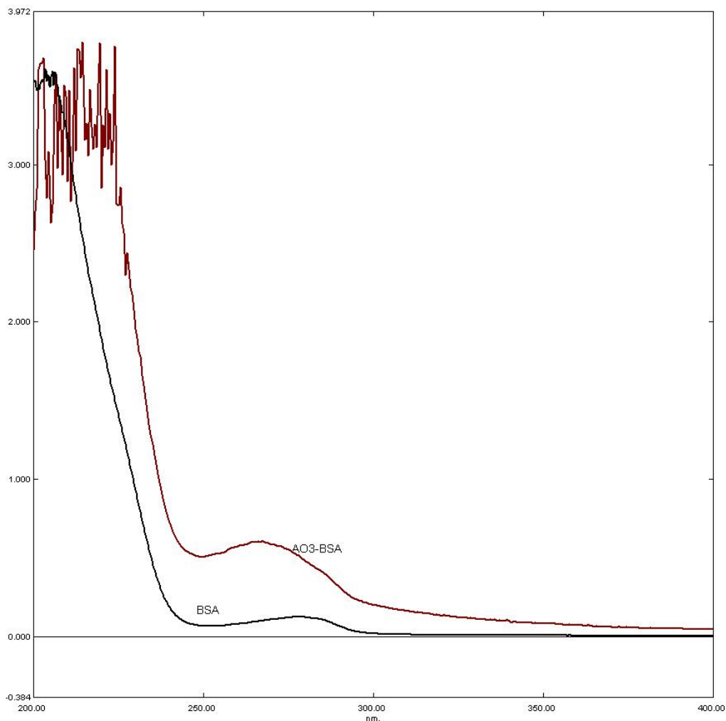
Figure 2. UV-spectrum
