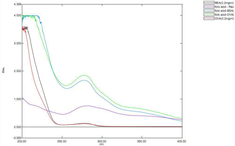
Figure 1. UV-spectrum
