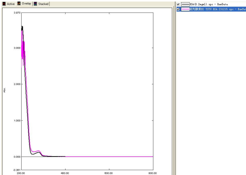
Figure . UV-spectrum
