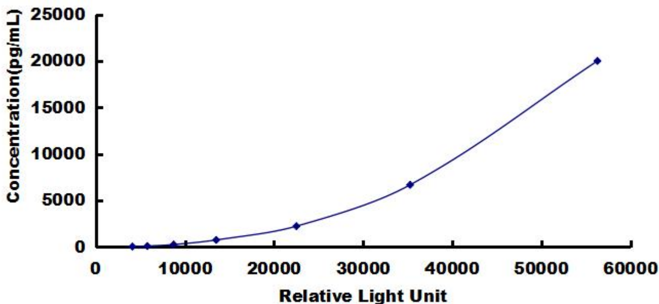
Typical Standard Curve for ALOX12, Human CLIA.
