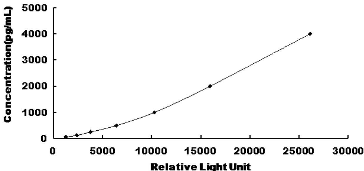
Typical Standard Curve for Human CNTF CLIA.
