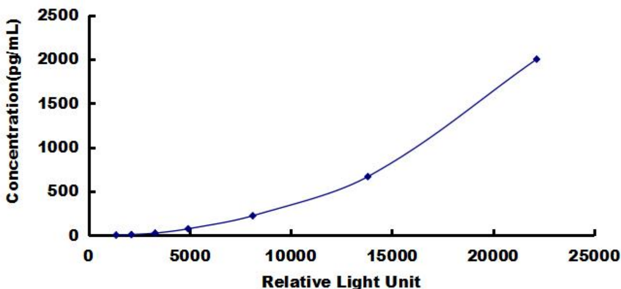
Typical Standard Curve for MIg, Human CLIA.
