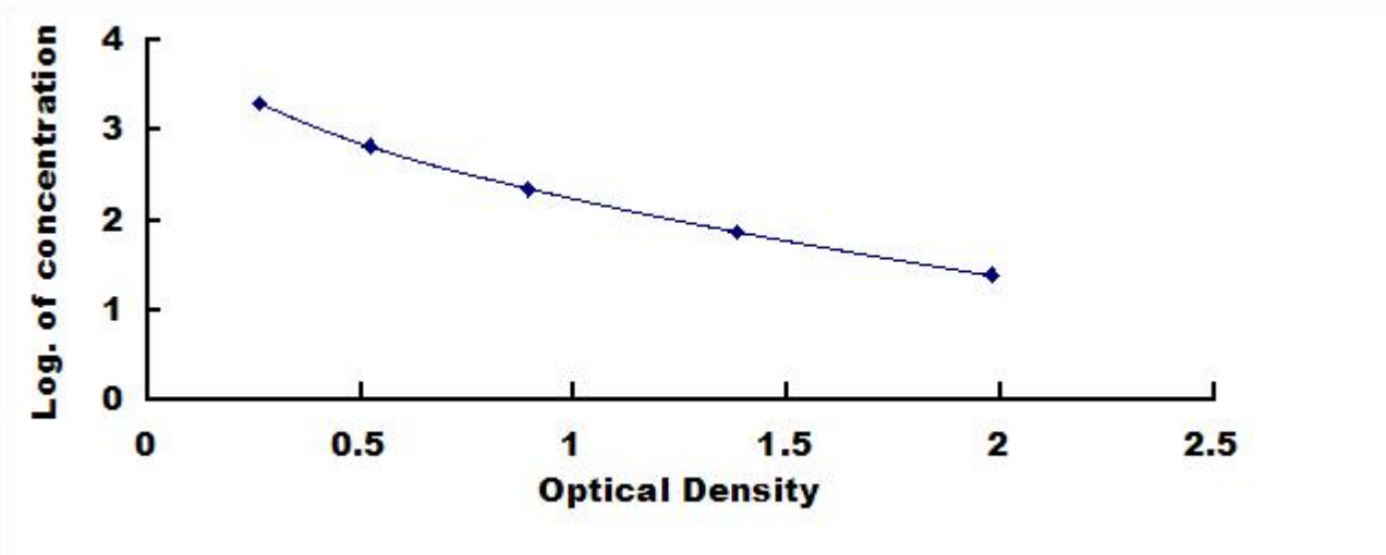
Typical Standard Curve for Angl, Canine ELISA.
