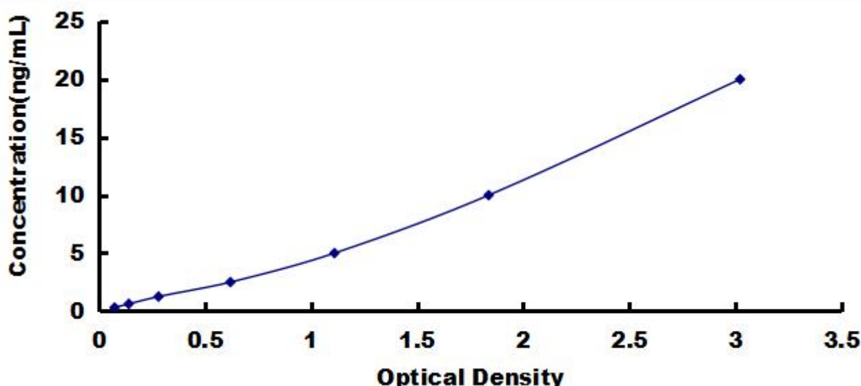
Typical Standard Curve for Anti-LCAT, Human ELISA.
