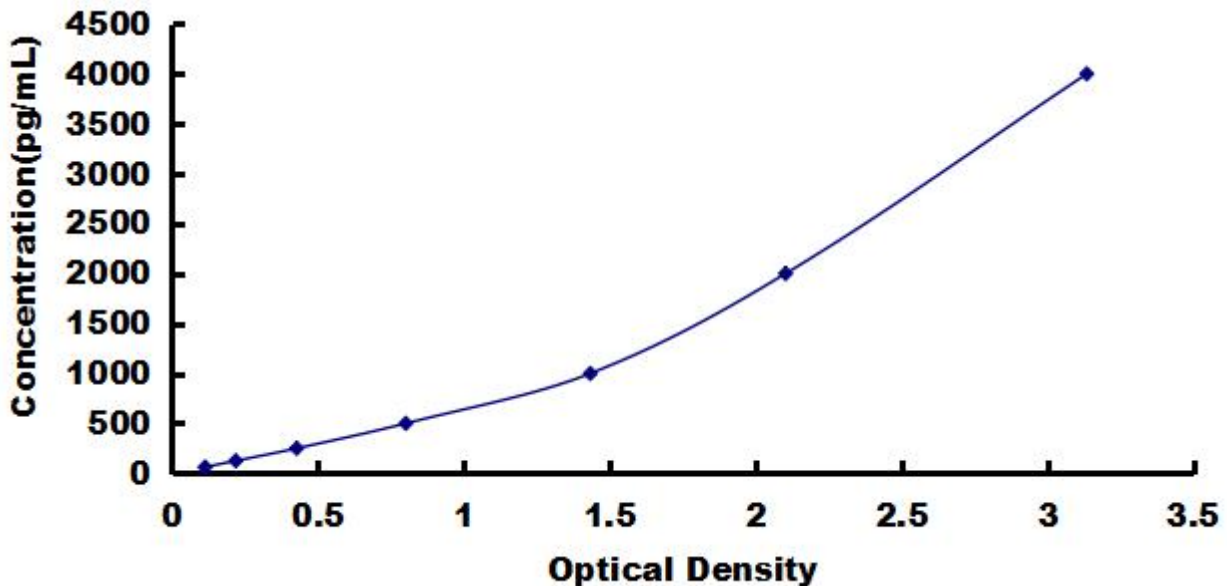
Typical Standard Curve for ASGR2, Human ELISA.
