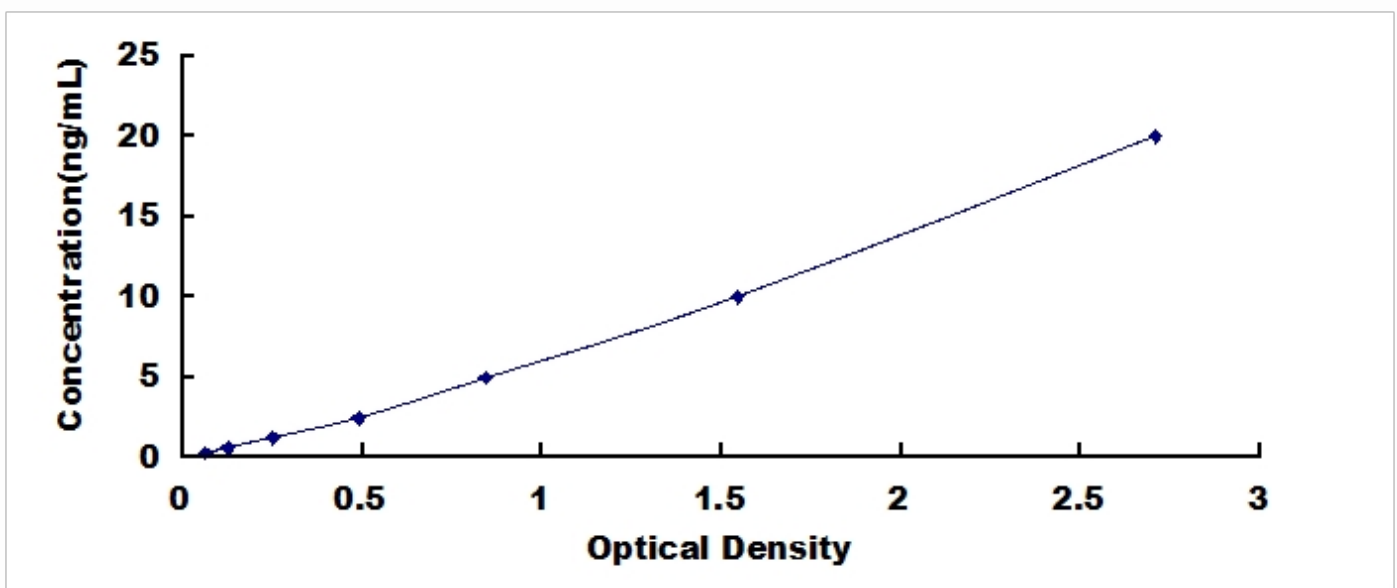
Typical Standard Curve for b2M, Rat ELISA.
