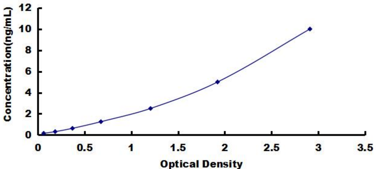
Typical Standard Curve for CASP3, Bovine ELISA.
