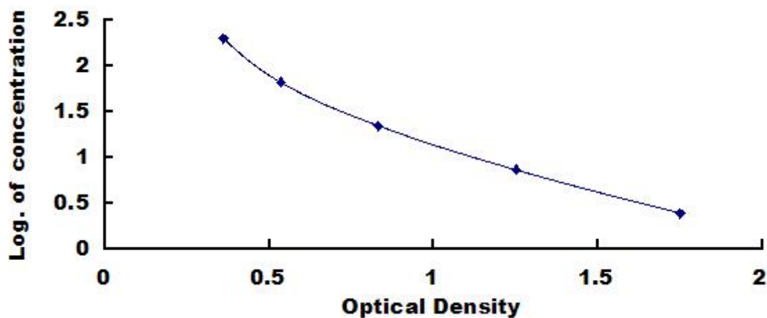
Typical Standard Curve for NTXI, Rat ELISA.
