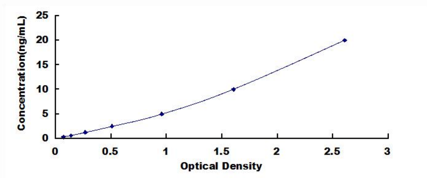
Typical Standard Curve for CYP3A2, Rat ELISA.
