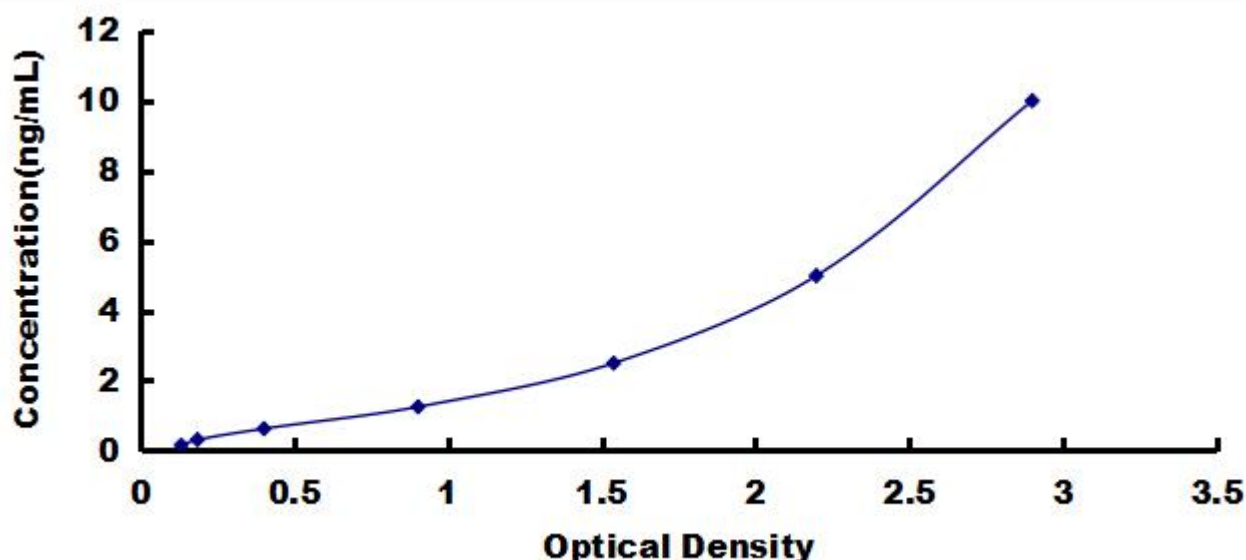
Typical Standard Curve for DISC1, Human ELISA.
