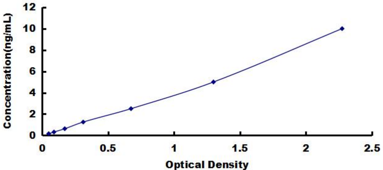
Typical Standard Curve for DRD1, Mouse ELISA.
