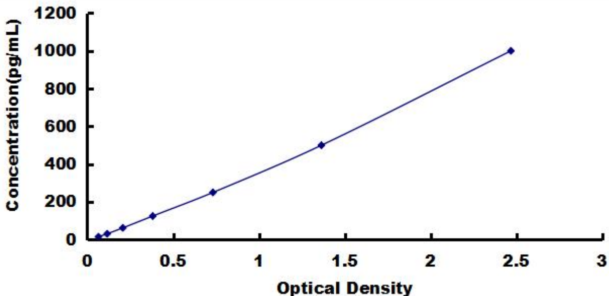
Typical Standard Curve for GDF15, Rat ELISA.
