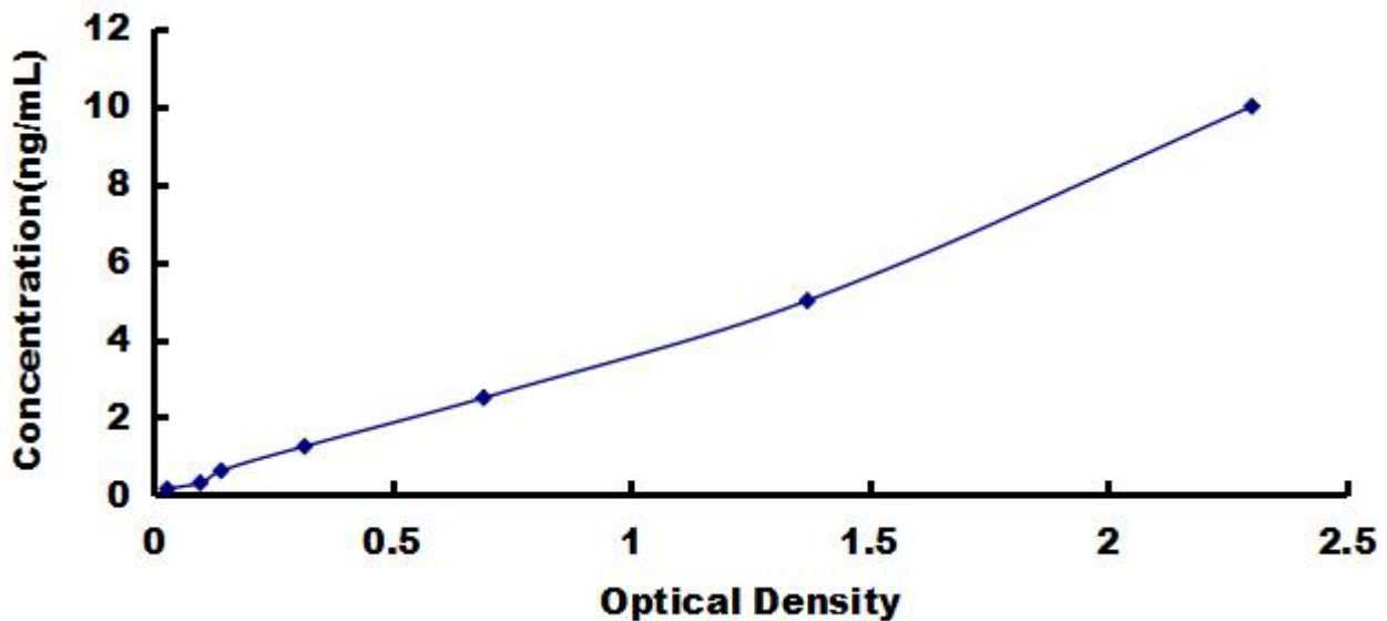
Typical Standard Curve for GUCA2B, Mouse ELISA.
