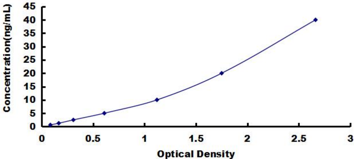
Typical Standard Curve for FABP3, Porcine ELISA.
