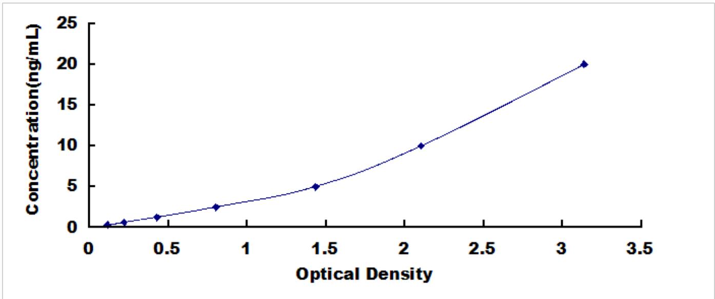
Typical Standard Curve for HO1, Human ELISA.
