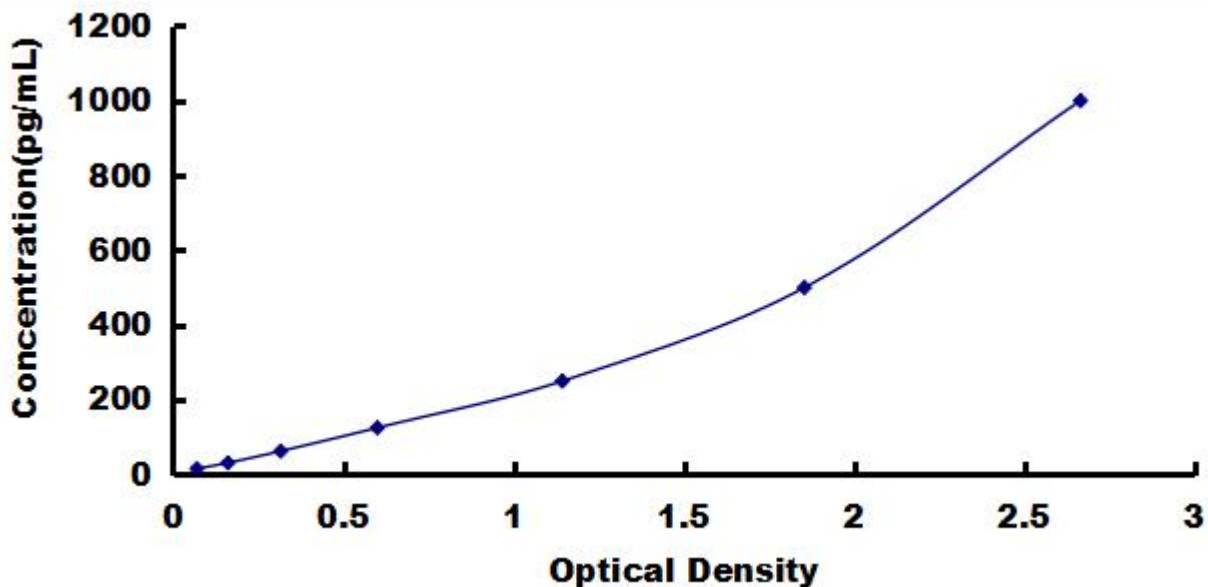
Typical Standard Curve for IFN̢, Canine ELISA.
