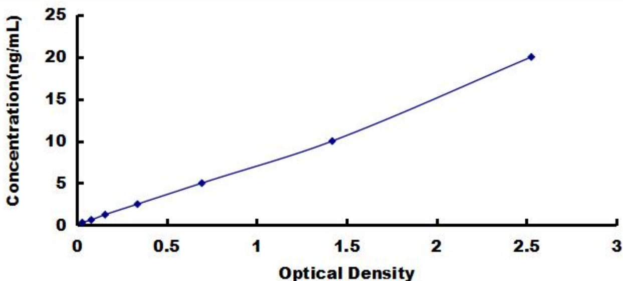
Typical Standard Curve for Leptin, Canine ELISA.
