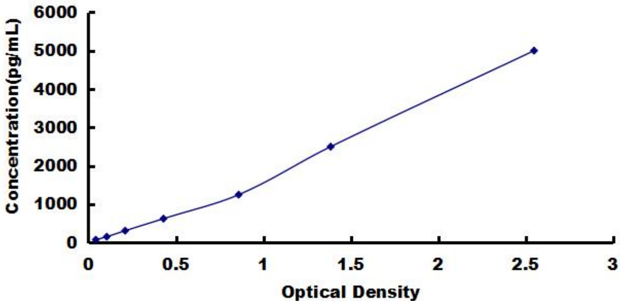
Typical Standard Curve for MIP1b, Rat ELISA.
