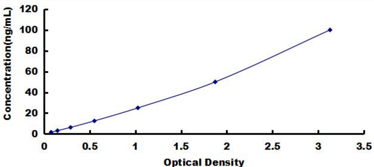
Typical Standard Curve for MMP13, Bovine ELISA.
