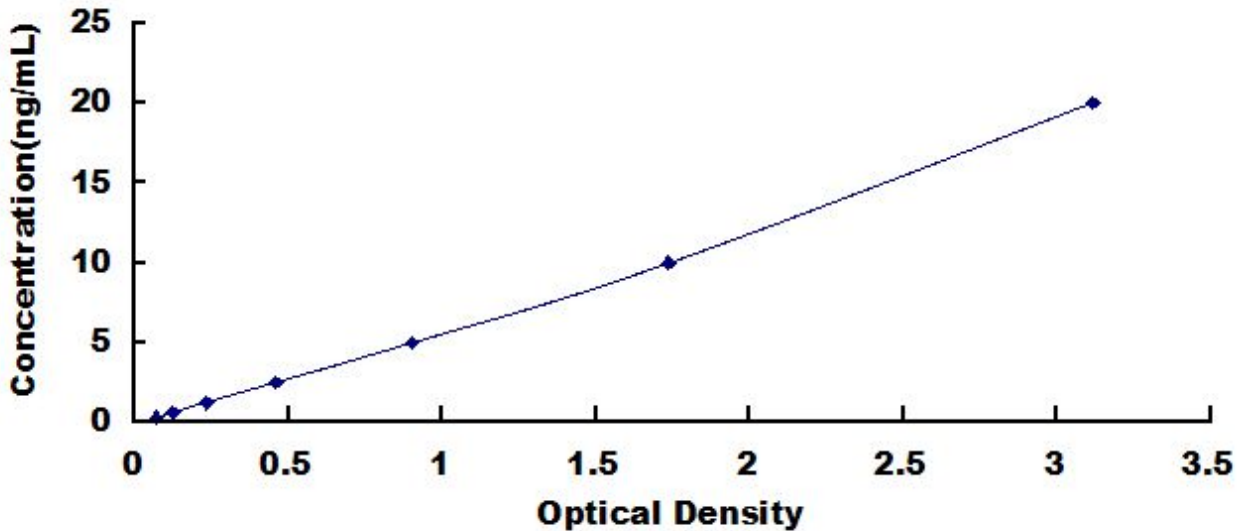
Typical Standard Curve for NRN1, Human ELISA.
