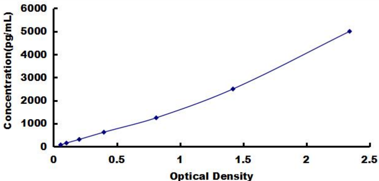
Typical Standard Curve for PENK, Mouse ELISA.
