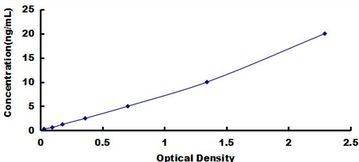
Typical Standard Curve for PKIa, Human ELISA.
