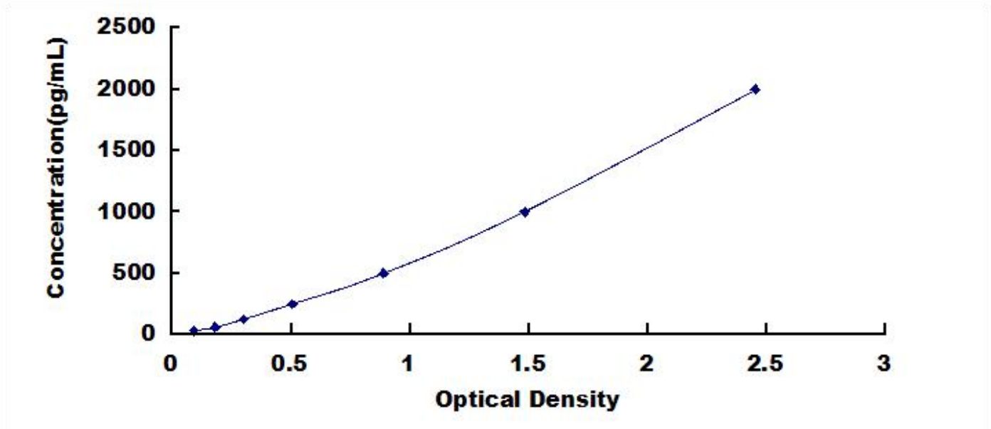
Typical Standard Curve for Renin, Canine ELISA.
