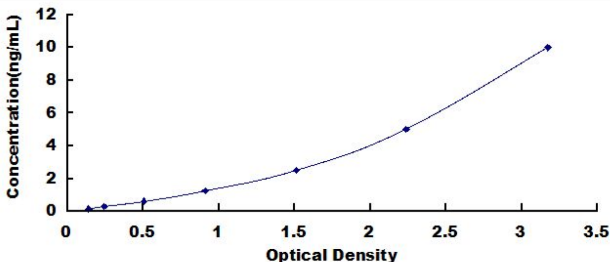
Typical Standard Curve for SCARB1, Mouse ELISA.
