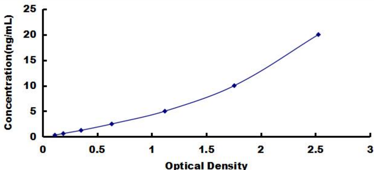
Typical Standard Curve for SLAMF1, Human ELISA.
