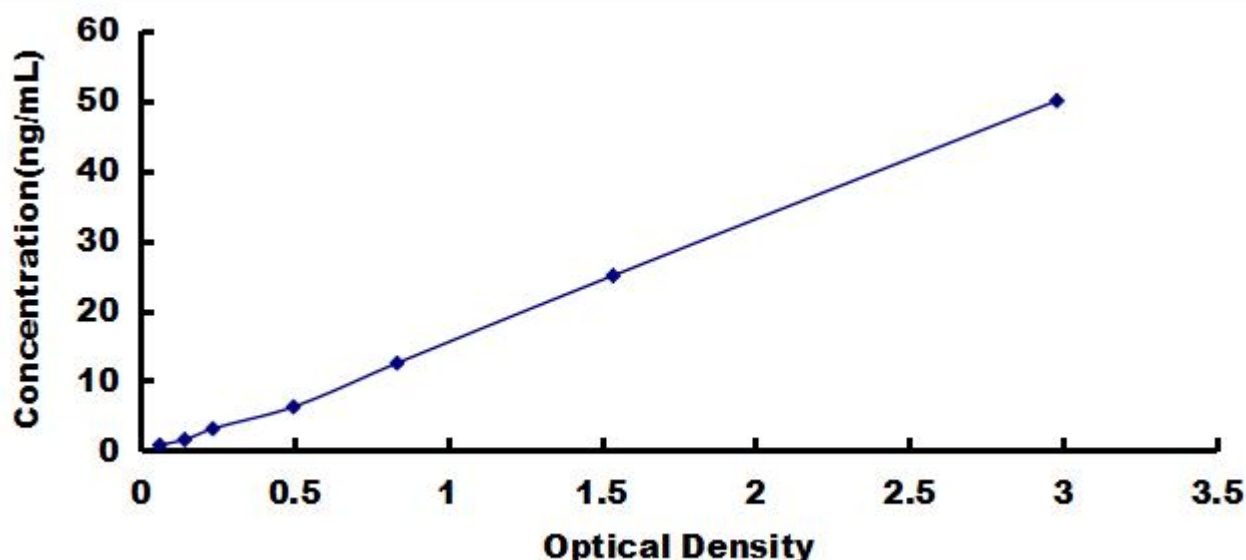
Typical Standard Curve for SSA1, Mouse ELISA.
