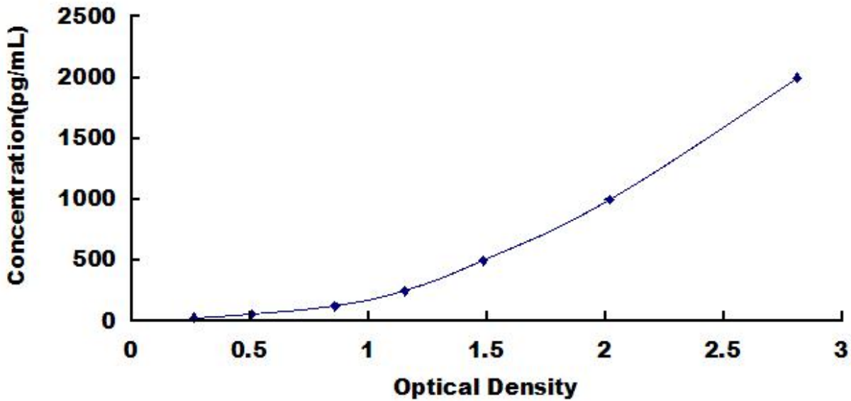
Typical Standard Curve for SULF2, Human ELISA.
