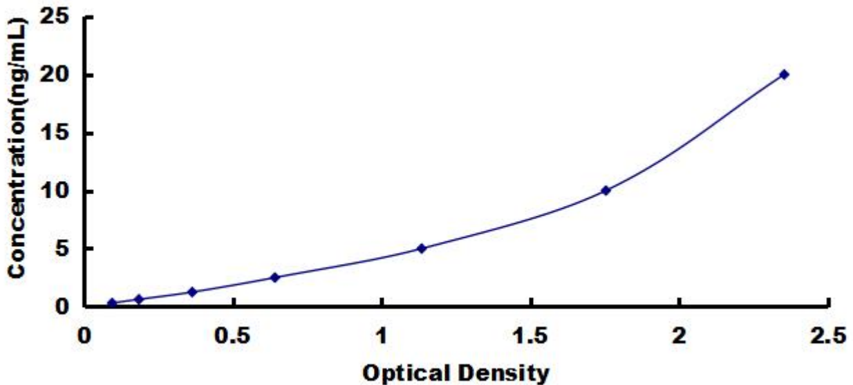
Typical Standard Curve for TIC2, Human ELISA.
